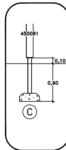
Sunken Foundation
